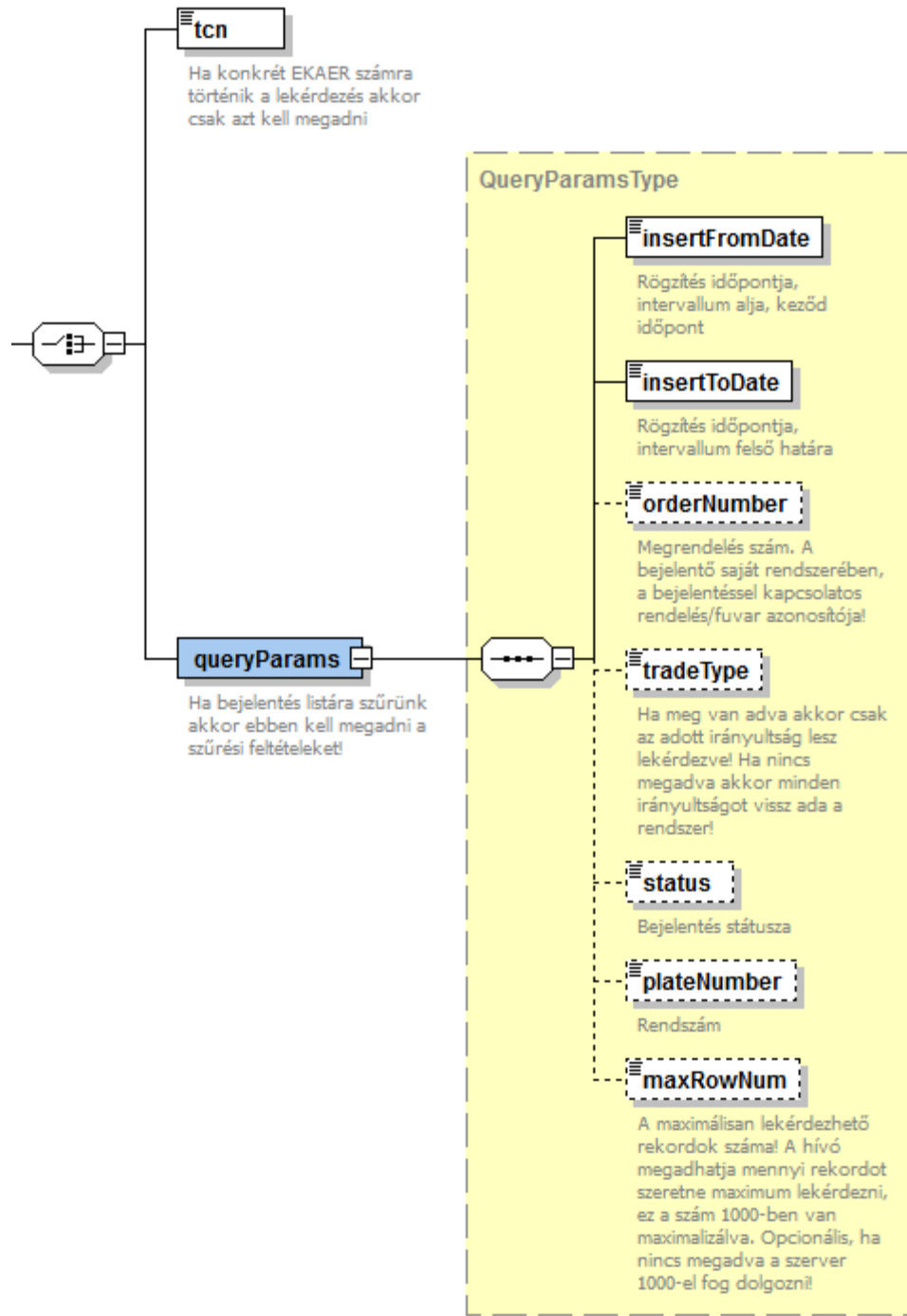
6. illustration queryTradeCardsRequest condition choice structure
