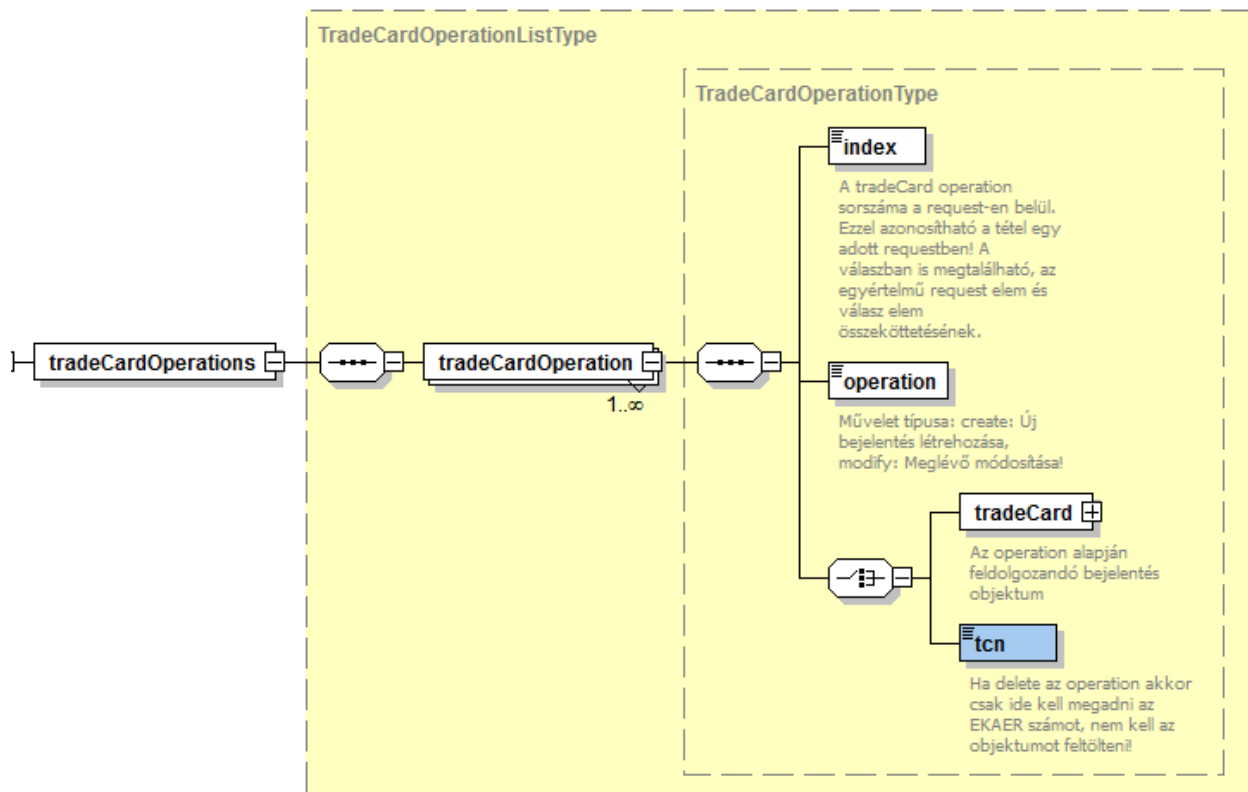
3. illustration tradeCardOperation element structure
