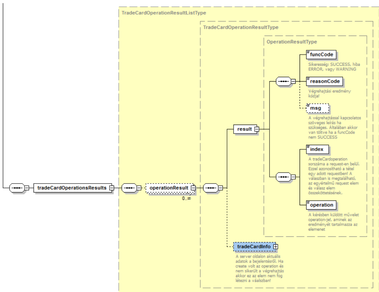
5. Illustration tradeCardOperationsResults structure
